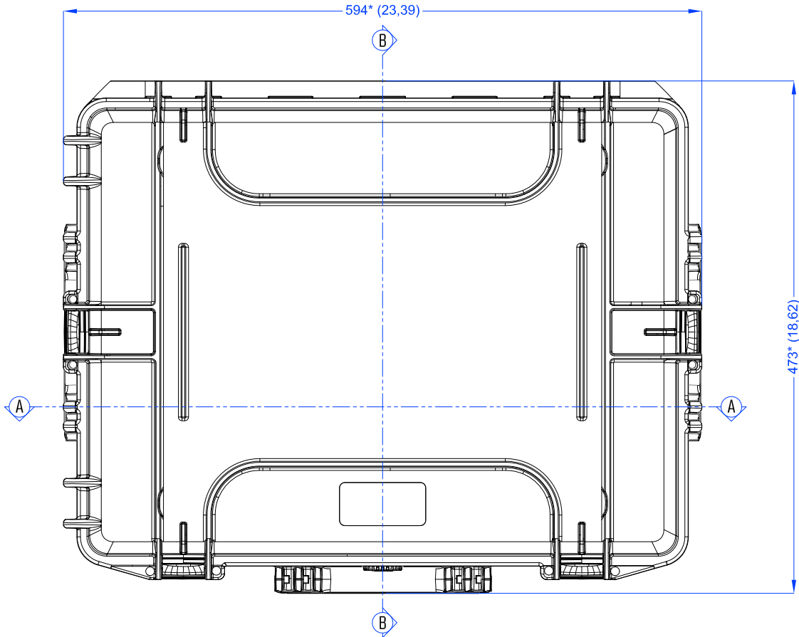
Vista Coperchio Lid View
